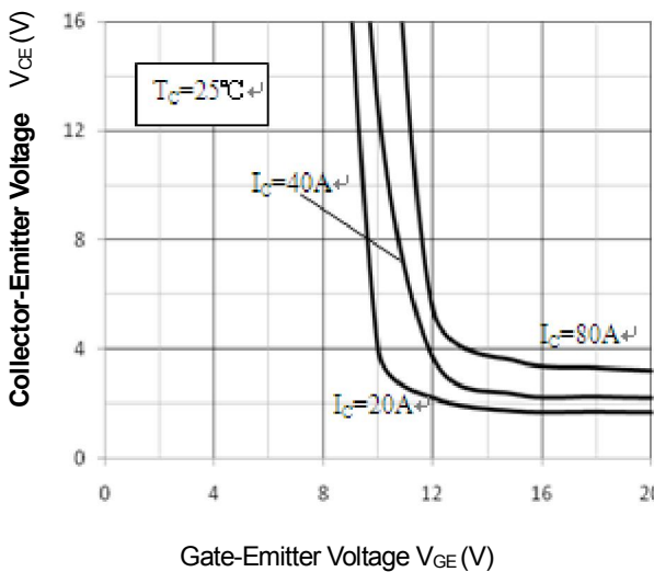
Figure 5. V_{CE(sat)} - V_{GE} Characteristics
